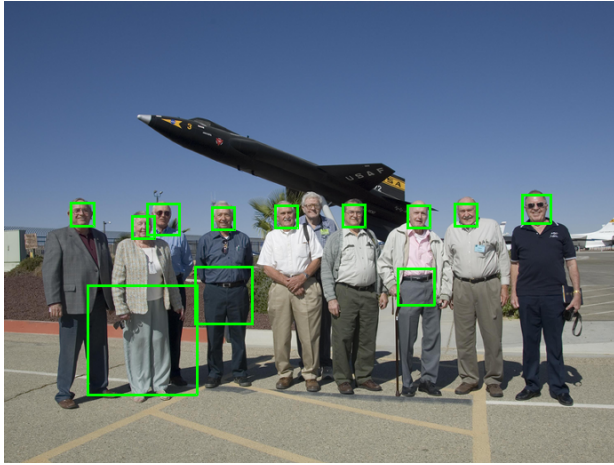
NFP_{\max} = 100
