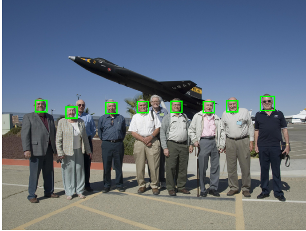
NFP_{\max} = 1
