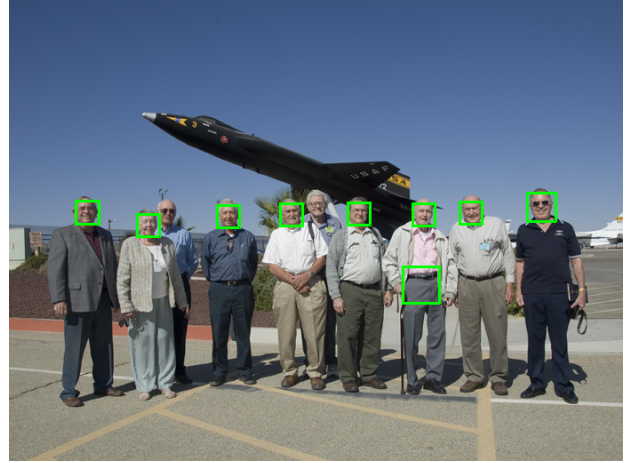
NFP_{\max} = 10
