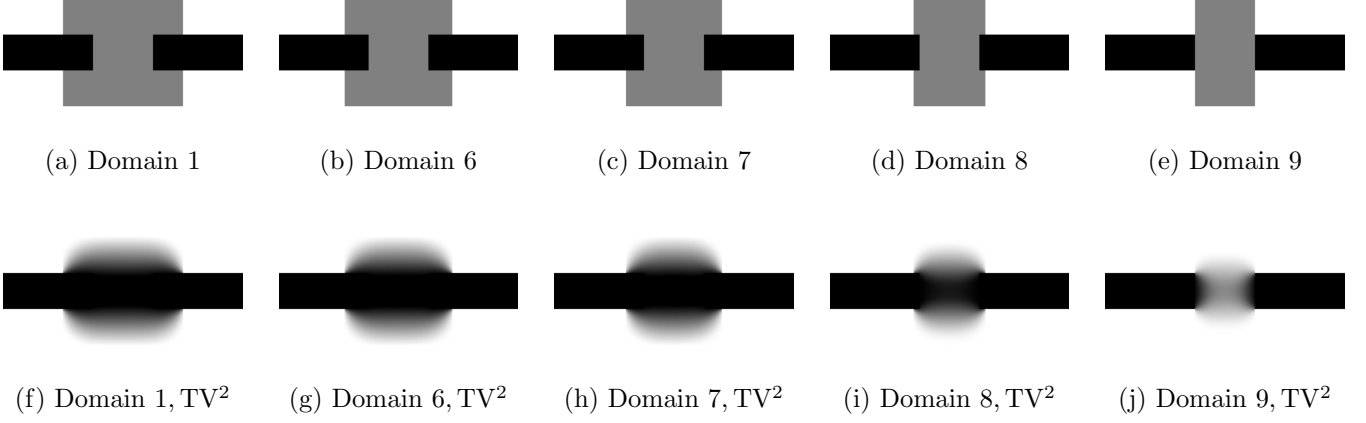
Figure 11: Different pure \text{TV}^2 inpainting results for different inpainting domains of decreasing width. In all computations we set \beta = 0.001 .
