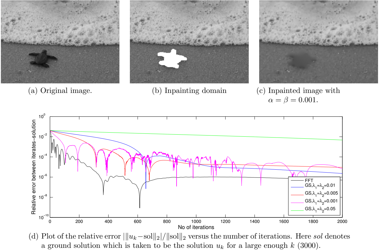
Figure 5: We compare the efficiency of the fast Fourier transform for the solution of (18) and one iteration of Gauss–Seidel for the solution of (24). For the FFT the choice of \lambda 's is done according to (44) while for the Gauss–Seidel the selection of \lambda 's is shown in figure (d). We observe that solving the linear subproblem with FFT leads to a faster convergence as figure (d) suggests. Using more than one iterations of Gauss–Seidel do not improve the situation significantly and also increase the computational time, see also the corresponding discussion in Goldstein and Osher [16].
