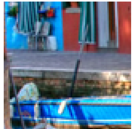
\sigma = 5, A_{YCbCr}
