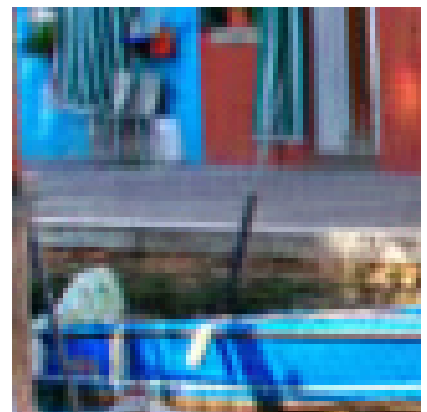
\sigma = 15, A_{YCbCr}
