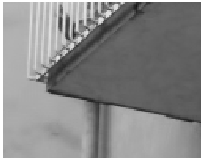
Basic estimate
