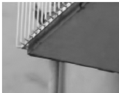
Basic estimate
