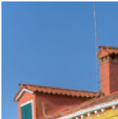
\sigma = 5, A_{YUV}
