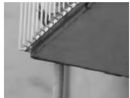
Final estimate
