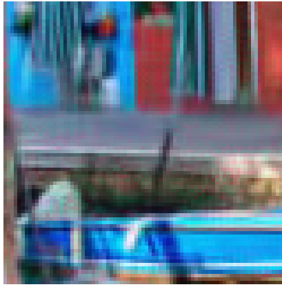
\sigma = 30, A_{YUV}
