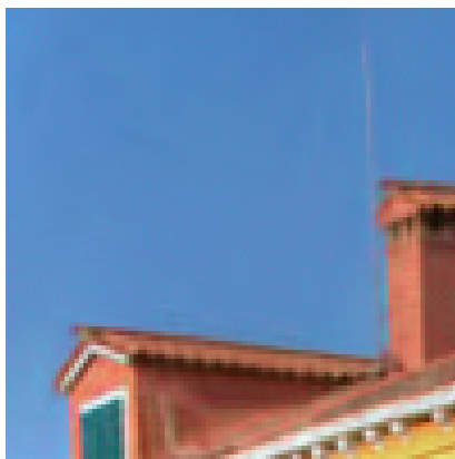
\sigma = 15, A_{YUV}
